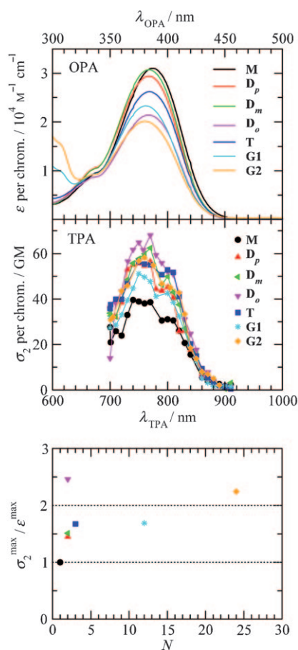
Figure 1. Top panels: experimental OPA and TPA per chromophoric subunit, measured in dimethyl sulfoxide (DMSO) solution. Bottom panel: the \sigma_2^{\text{max}}/\sigma_1^{\text{max}} ratio as a function of the number N of chromophoric subunits.
