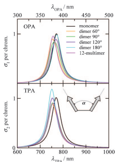
Figure 2. Calculated OPA and TPA per chromophoric subunit for monomer, dimers of varying interchromophore angle ( \alpha , see legend and inset), and a 12-chromophore multimer of icosahedral symmetry. The exciton coupling was fixed to \sum_{j \neq i} J_{ij} = 0.05 \text{ eV} .
